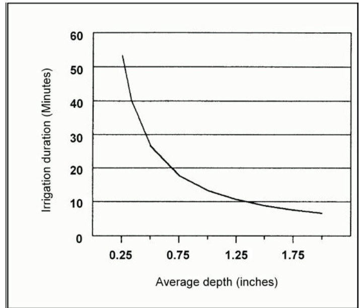
Figure 8. Time that an irrigation system should be on to apply \frac{2}{3} of an inch of water to a soil that has been depleted 50%.
