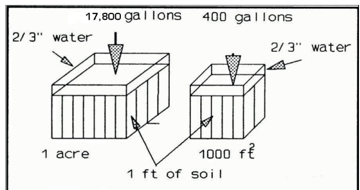
Figure 6. Irrigation volumes required for different size areas to replenish a soil ( 1''/\text{ft} SWHC) depleted to 50% using an impact sprinkler.
