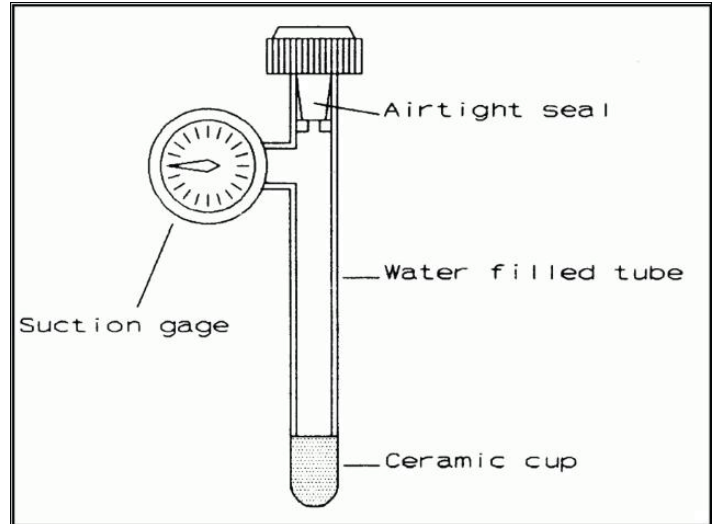
Figure 5. Tensiometer.
