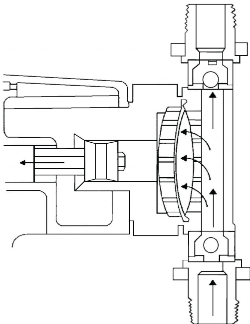
Figure 4a. Diaphragm pump - suction stroke.
