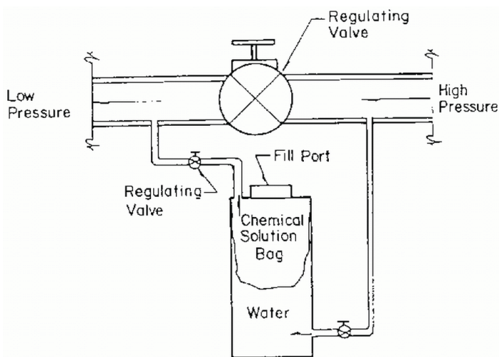
Figure 12. Proportional mixer.
