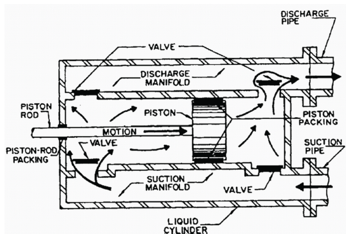
Figure 6. Double acting piston pump.
