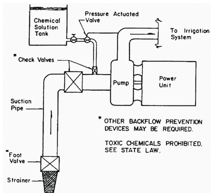
Figure 10. Suction line injection.
