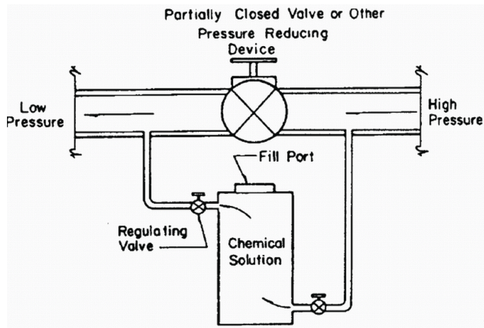
Figure 11. Pressurized mixing tank.
