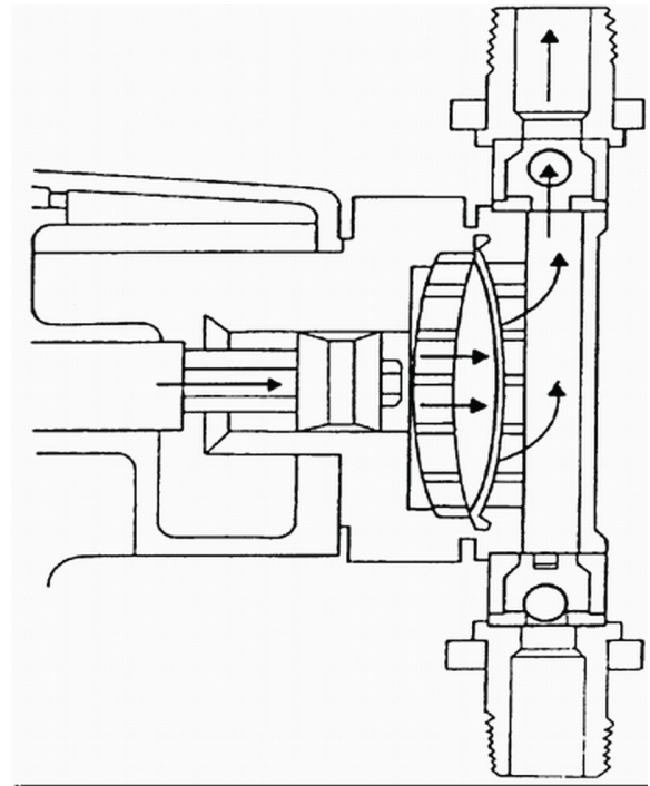
Figure 4b. Diaphragm pump - discharge stroke.
