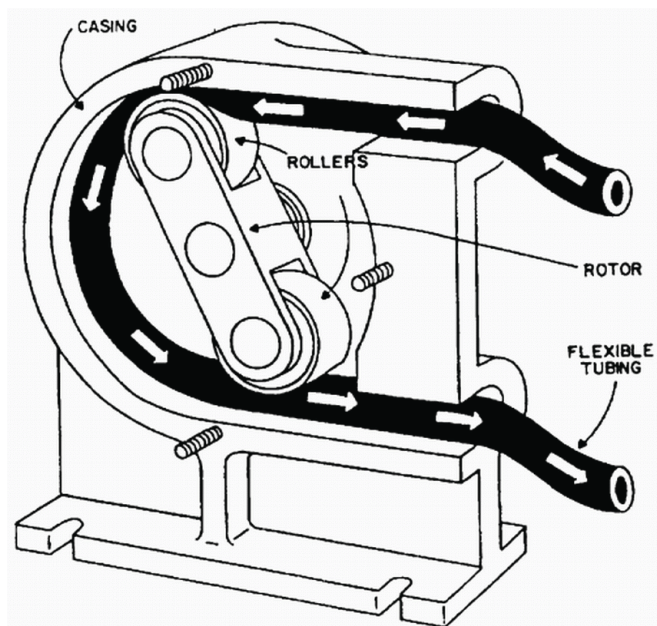
Figure 9. Peristaltic pump.
