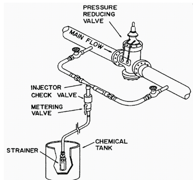
Figure 14. Small venturi injector with regulator valve for pressure drop in the main line.
