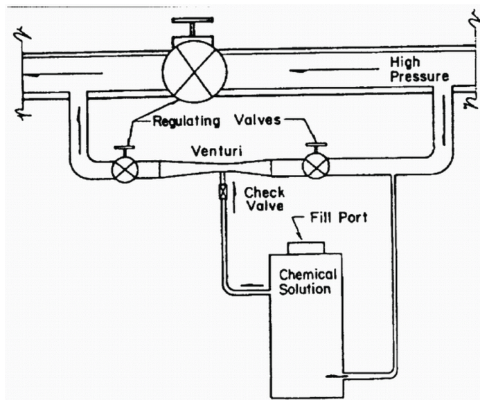
Figure 16. Combination of a pressurized tank and venturi injector.
