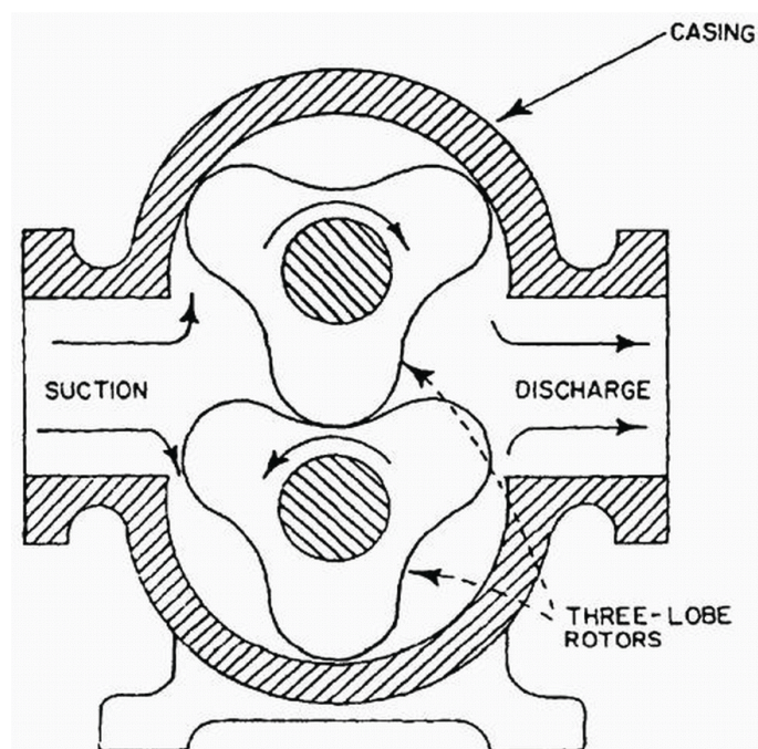
Figure 8. Lobe pump.
