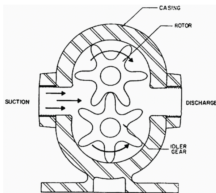
Figure 7. Gear pump.
