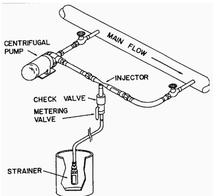
Figure 15. Small venturi injector in conjunction with a centrifugal booster pump.
