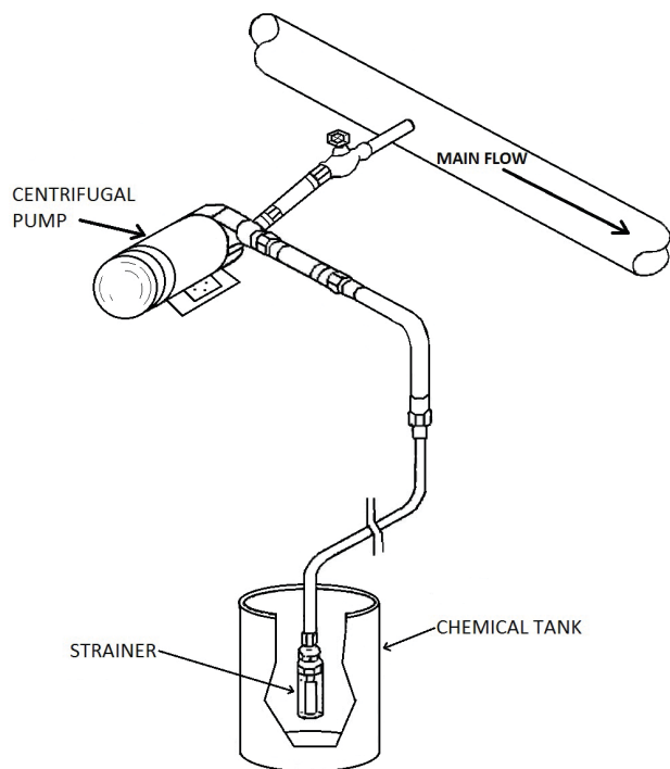
Figure 2. Centrifugal pump chemical injector.
