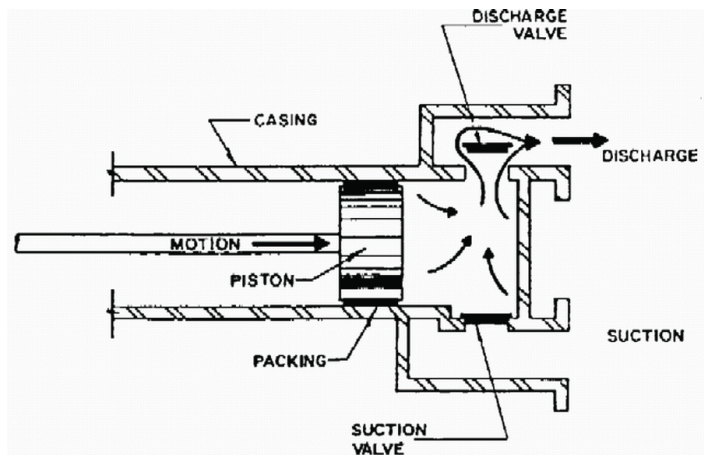
Figure 3b. Piston pump - discharge stroke.
