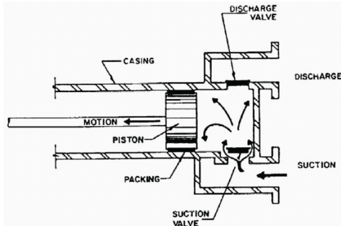
Figure 3a. Piston pump - suction stroke.
