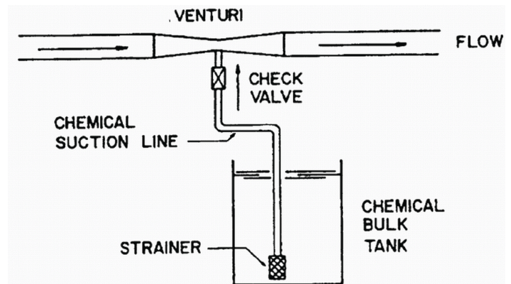
Figure 13. Venturi injector in the main line.
