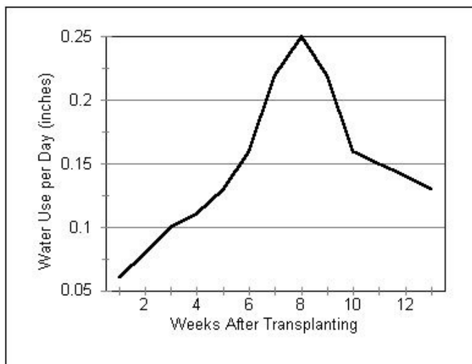
Fig. 1. Moisture Use by Tobacco (Harrison and Whitty, 1971)
